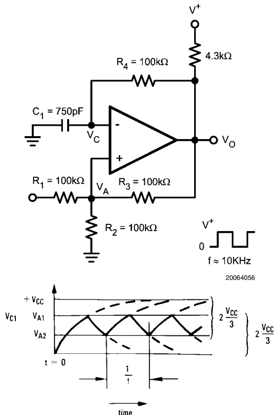
FIGURE 10. Squarewave Oscillator
