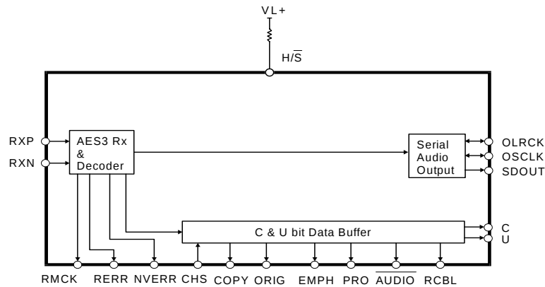
Figure 9. Hardware Mode
