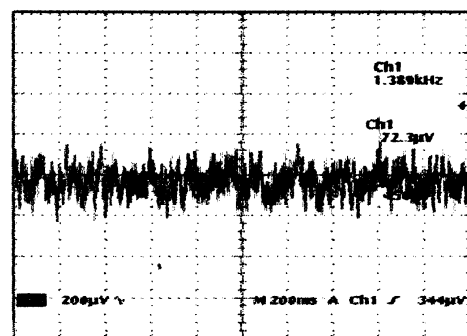
Output Noise DC to 1MHz
