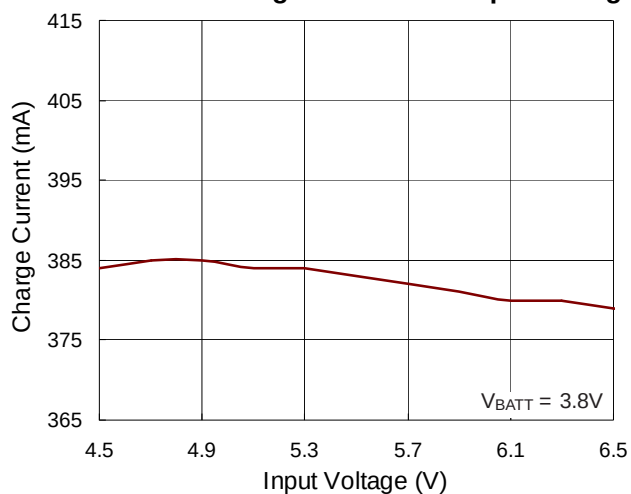
USB 500 Mode Charge Current vs. Input Voltage
