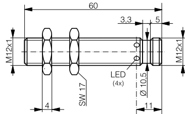
DW-DS-605/6-M12
