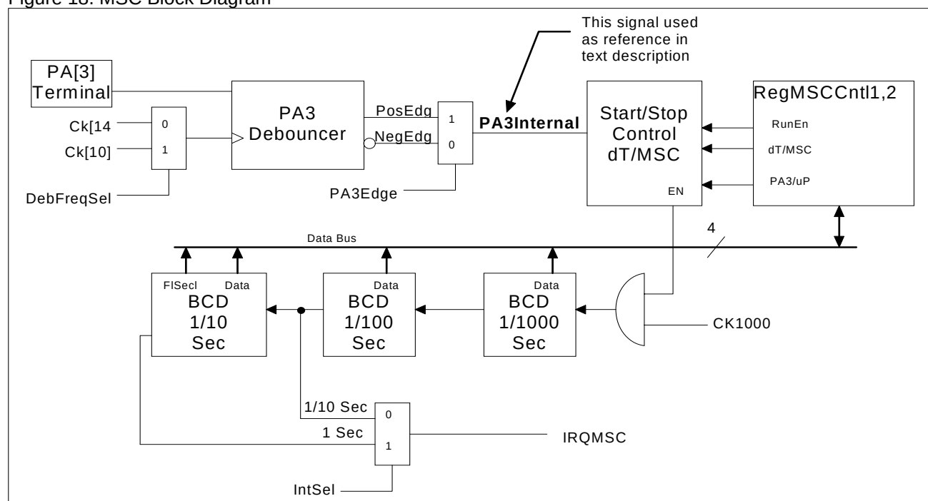
Figure 18. MSC Block Diagram
