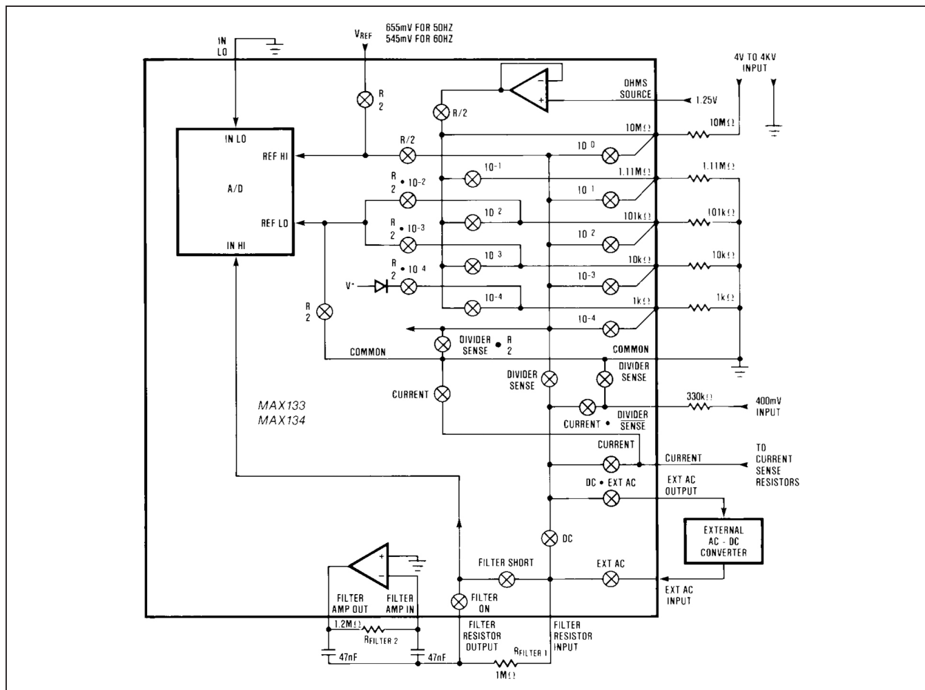
Figure 1. MAX133/134 Input Section
