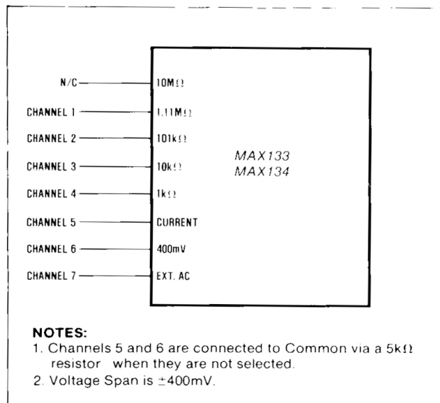
Figure 12. MAX133/134 Input Section used as a Multiplexer.
