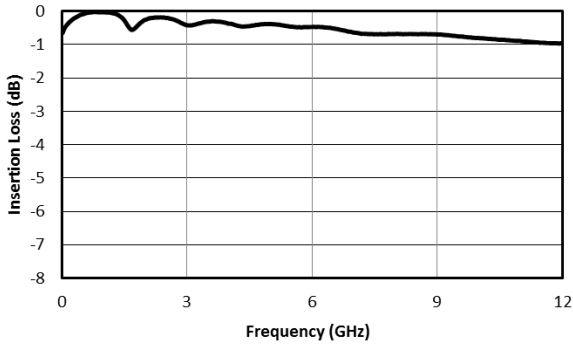
Fig. 1. Insertion loss.
