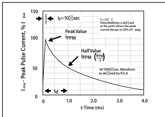
Figure 2. 10/1000μs Pulse Waveforms
