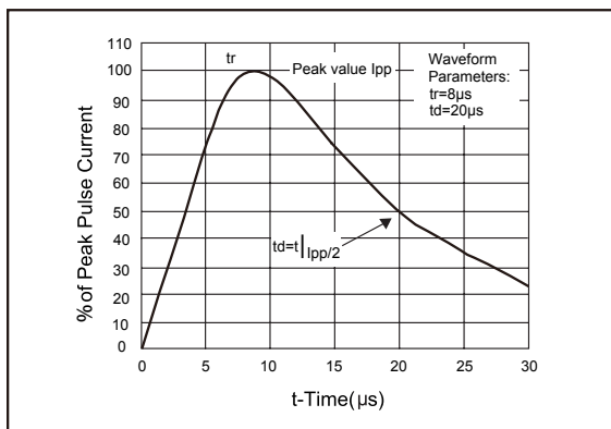
Figure 3. 8/20μs Pulse Waveforms
