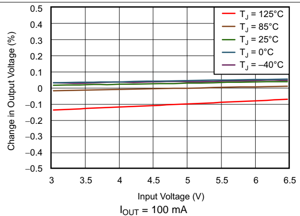
Figure 2. TPS73525 Line Regulation
