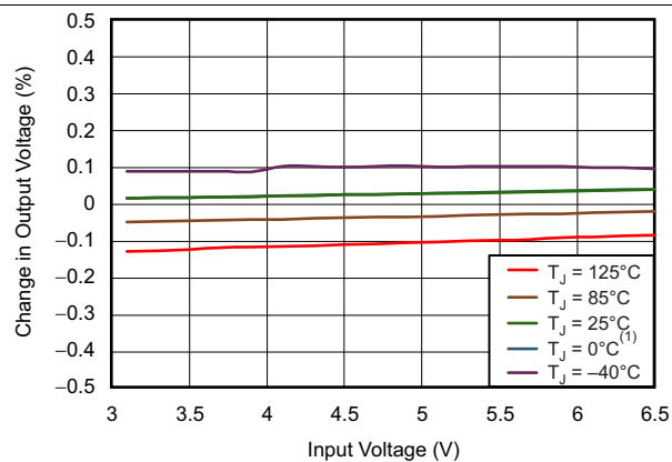
Figure 1. TPS73501 Line Regulation
