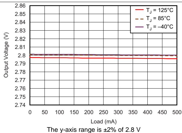
Figure 3. TPS73501 Load Regulation
