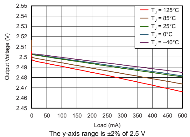
Figure 4. TPS73525 Load Regulation
