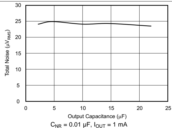
Figure 12. TPS73525 RMS Noise vs C_{OUT}
