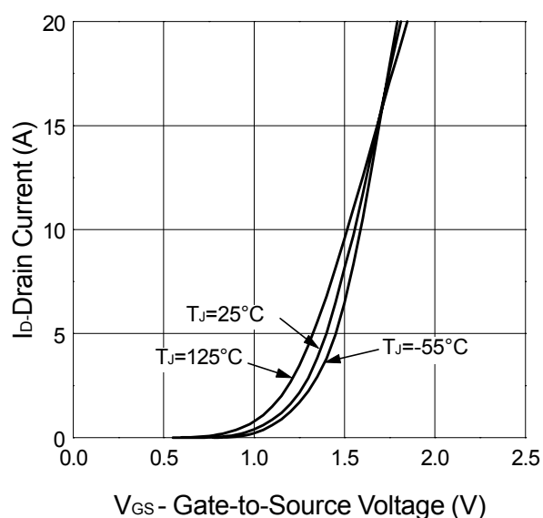
Transfer Characteristics
