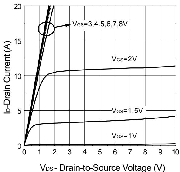
Output Characteristics
