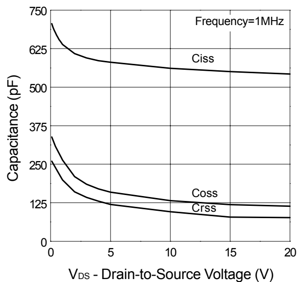
Capacitance
