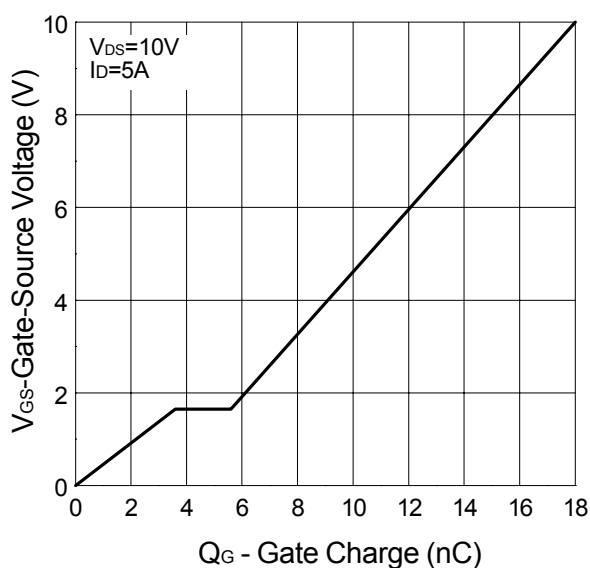
Gate Charge
