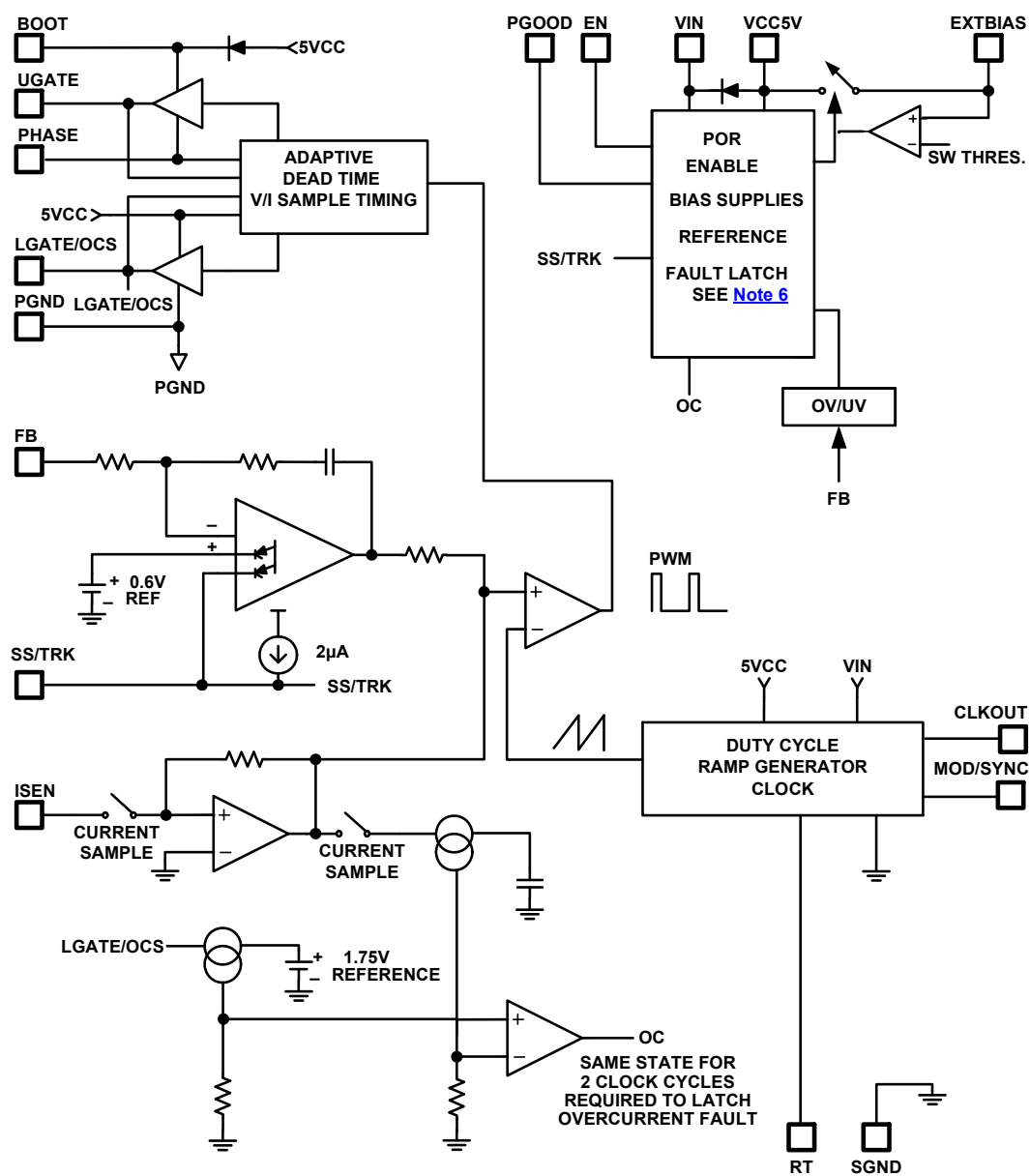
FIGURE 3. BLOCK DIAGRAM
