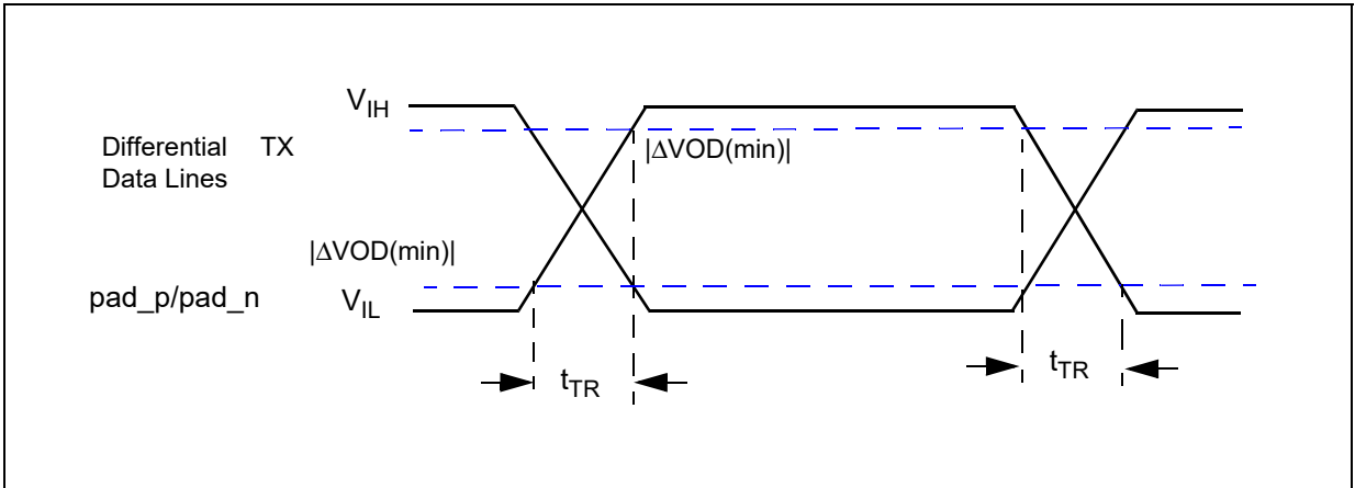
Figure 11. Rise/fall time
