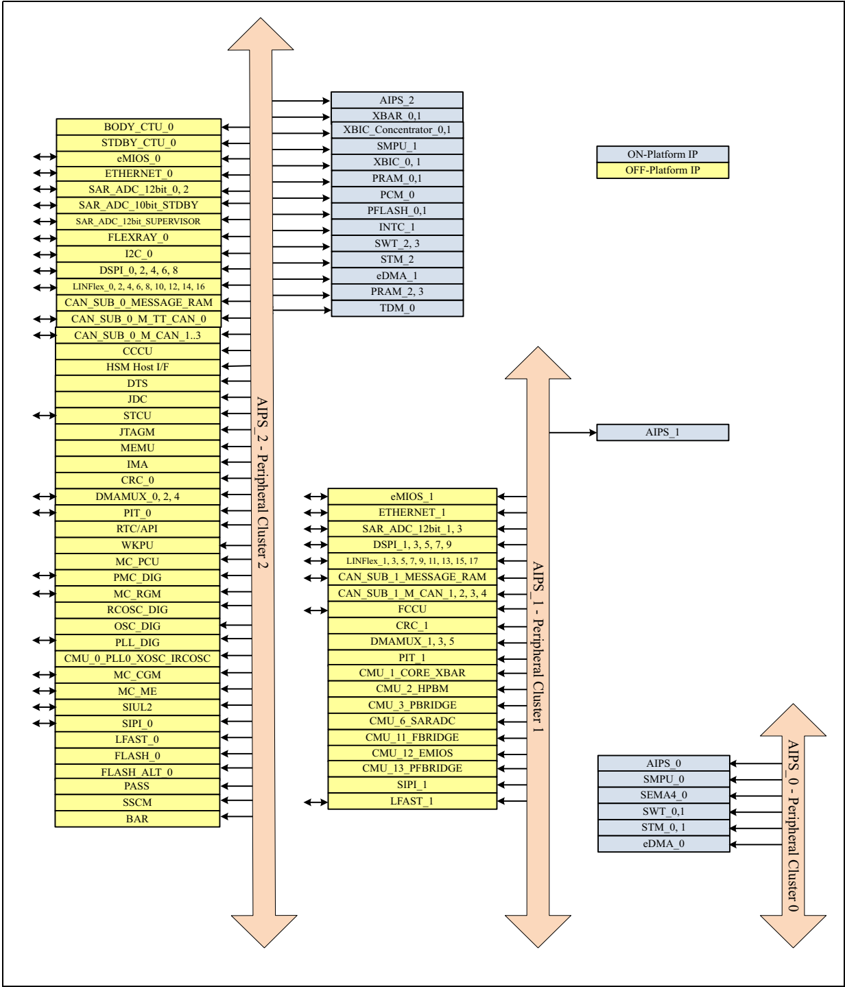
Figure 2. Peripheral allocation
