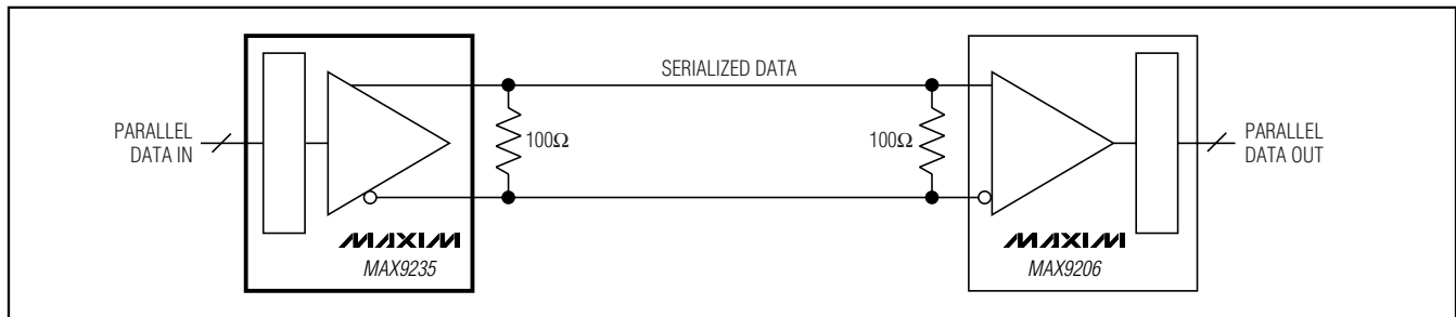
Figure 8. Double-Terminated Point-to-Point
