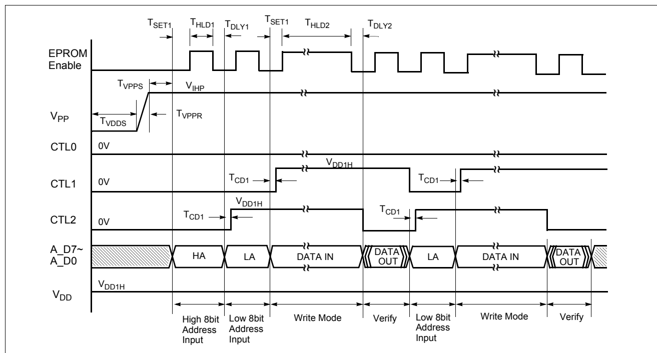
Figure 22-2 Timing Diagram in Program (Write &amp; Verify) Mode
