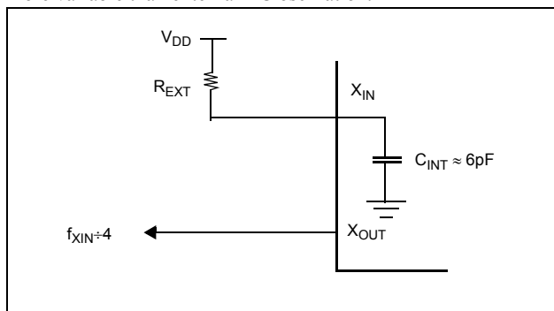
Figure 10-5 R Oscillator Connections
