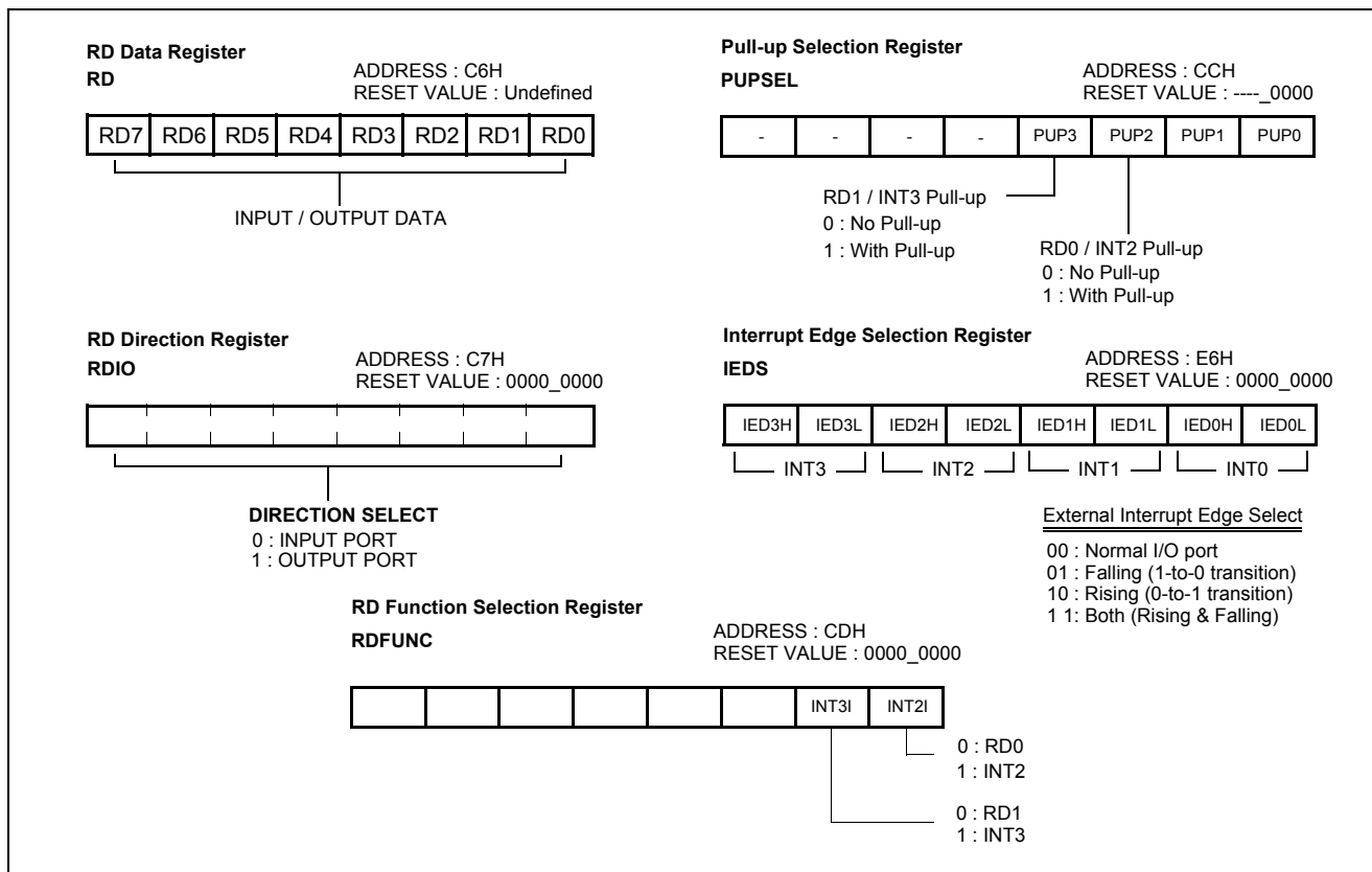
Figure 9-5 Registers of Port RD
