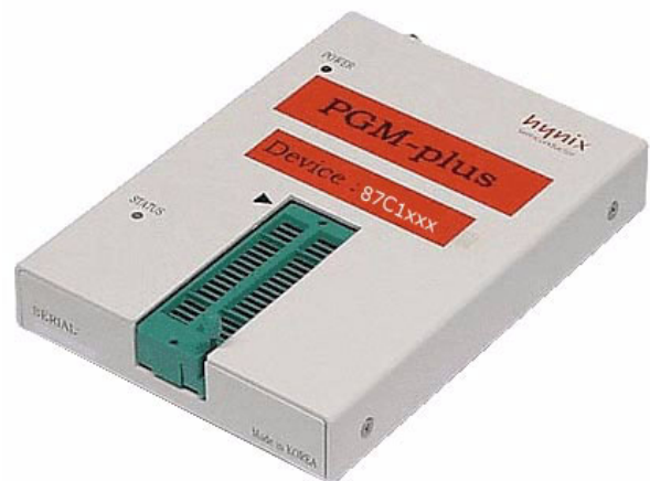
Figure 1-2 OTP Single Programmer PGM-plus™
