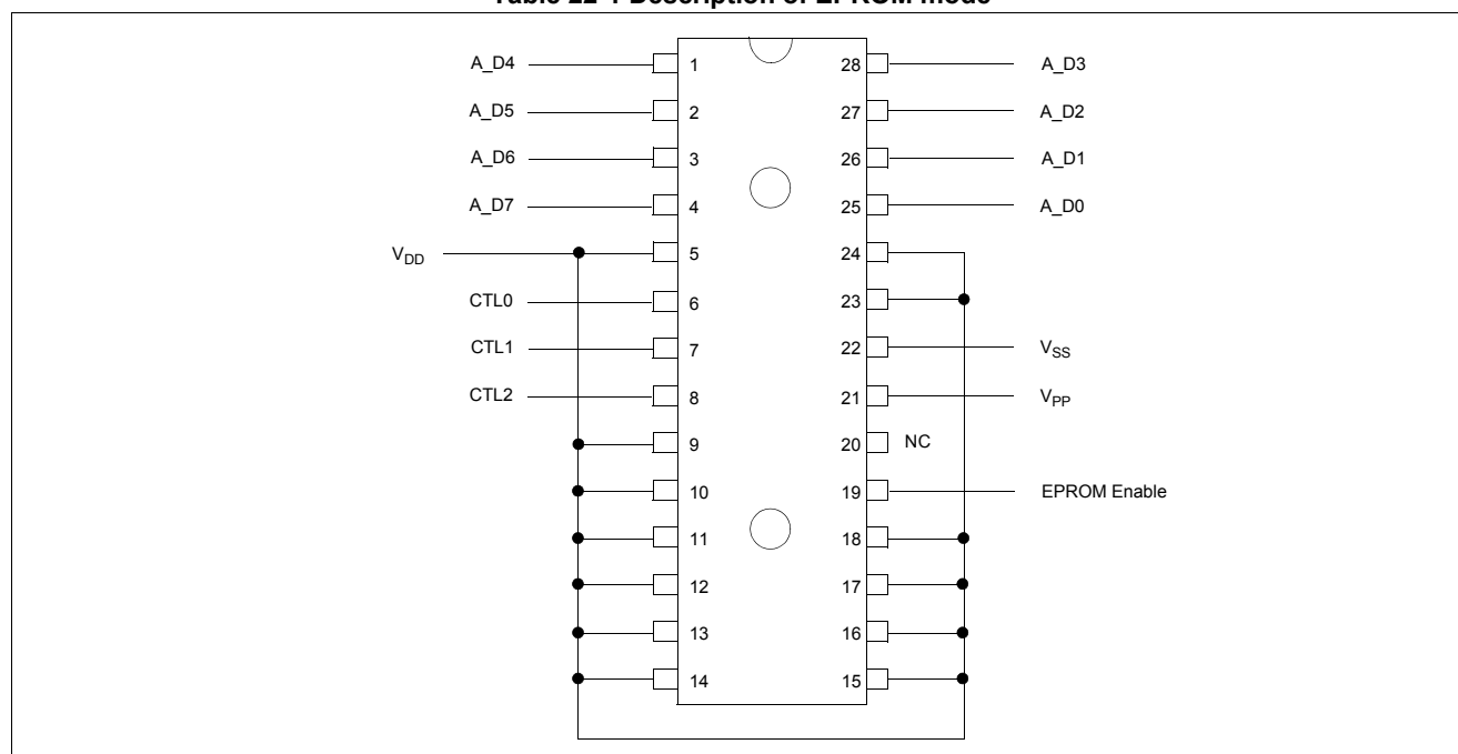
Figure 22-1 Pin Assignment
