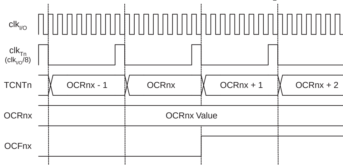
Figure 11-13. Timer/Counter Timing Diagram, Setting of OCF0x, with Prescaler ( f_{\text{clk\_I/O}}/8 )
