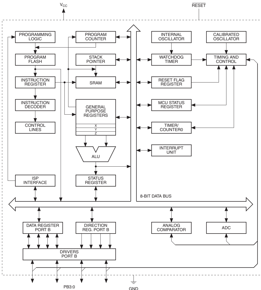
Figure 2-1. Block Diagram
