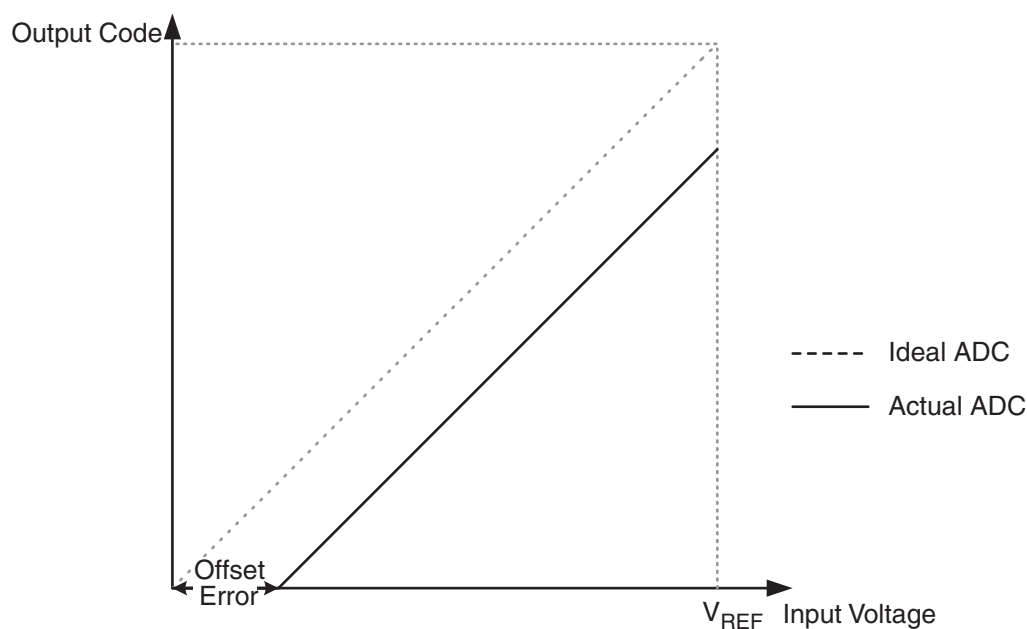
Figure 13-9. Offset Error
