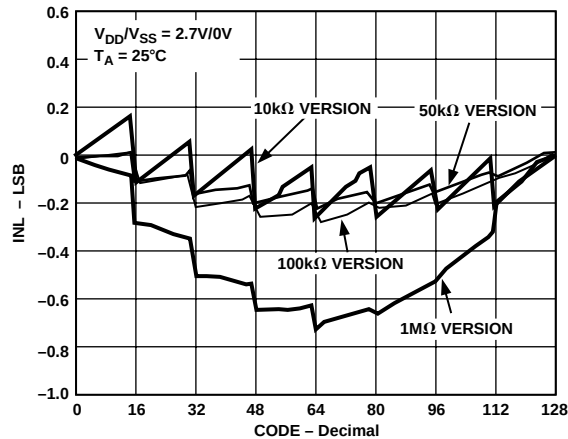
Figure 8. Potentiometer Divider INL Error vs. Code
