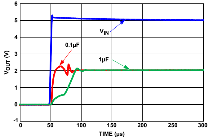
FIGURE 11. TURN-ON TIME
