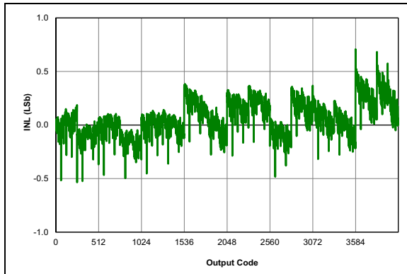
FIGURE 45-73: ADC 12-bit Mode, Single-Ended INL, V_{DD} = 3.0V , V_{REF} = 3.0V , T_{AD} = 1 \mu S , CP OFF, 25^{\circ}C .
