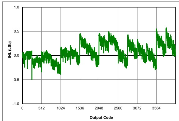
FIGURE 45-74: ADC 12-bit Mode, Single-Ended INL, V_{DD} = 3.0V , V_{REF} = 3.0V , T_{AD} = 1 \mu S , CP ON, 25^{\circ}C .
