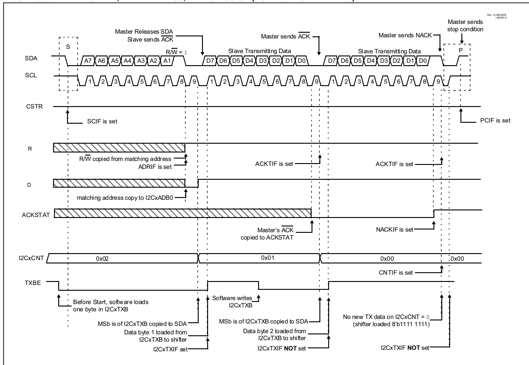
FIGURE 33-10: I 2 C SLAVE, 7-BIT ADDRESS, TRANSMISSION (NO CLOCK STRETCHING)
