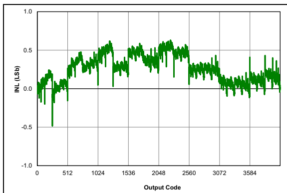
FIGURE 45-75: ADC 12-bit Mode, Single-Ended INL, V_{DD} = 2.3V , V_{REF} = 2.3V , T_{AD} = 1 \mu S , CP ON, 25^{\circ}C .
