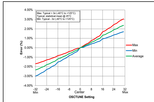
FIGURE 45-117: OSTUNE Center Frequency, PIC18LF24/25K42 Only.
