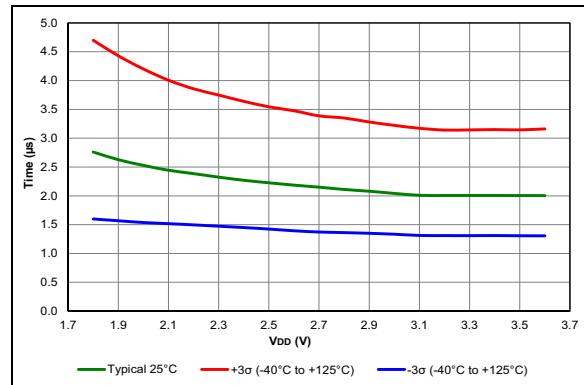
FIGURE 45-78: ADC RC Oscillator Period, PIC18LF24/25K42 Only.
