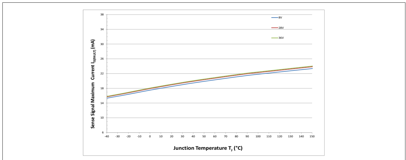
Figure 48 Sense Signal Maximum Current in Fault Condition I_{IS(FAULT)} = f(T_J; V_S)
