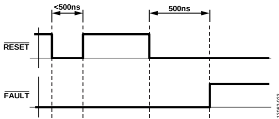
Figure 23. \overline{\text{RESET}} Timing
