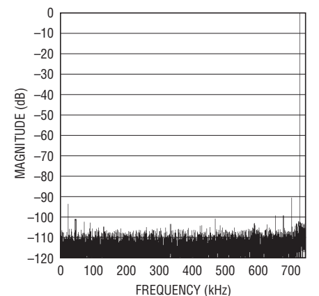
748kHz Sine Wave 4096 Point FFT Plot
