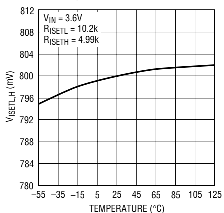
I_{\text{SETL,H}} Servo Voltage vs Temperature
