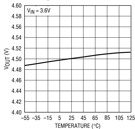
Maximum Regulated V_{\text{OUT}} vs Temperature
