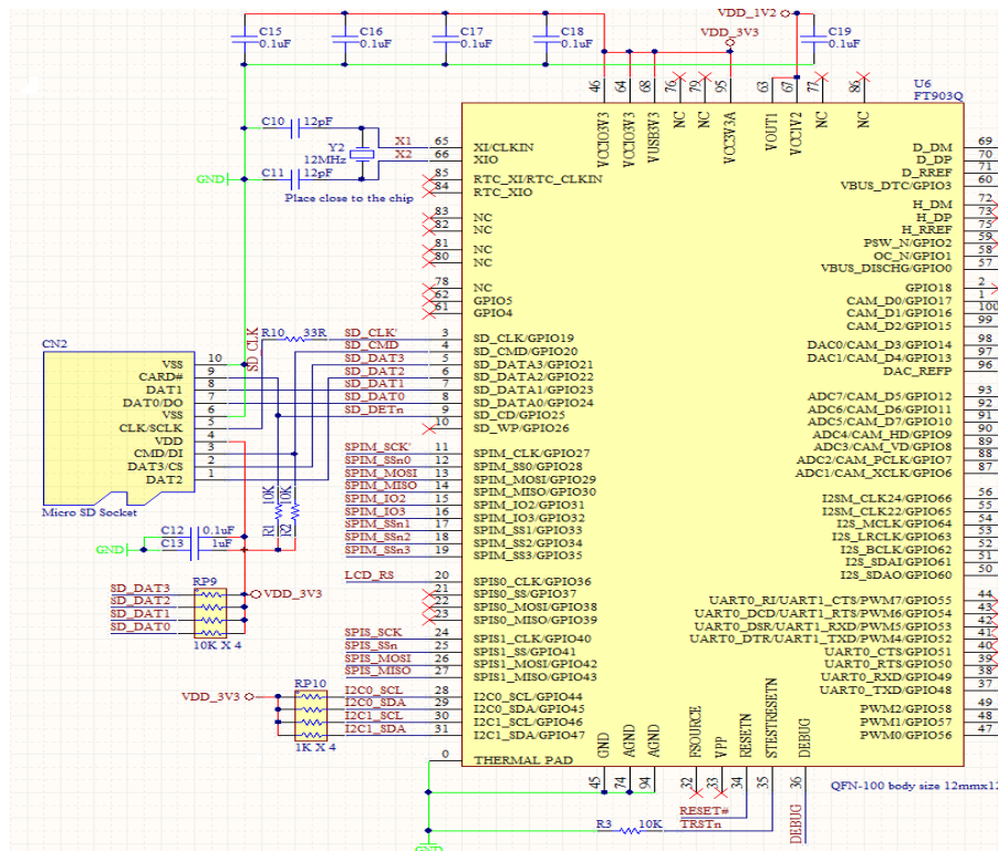
Figure 4 - MicroSD Interface
