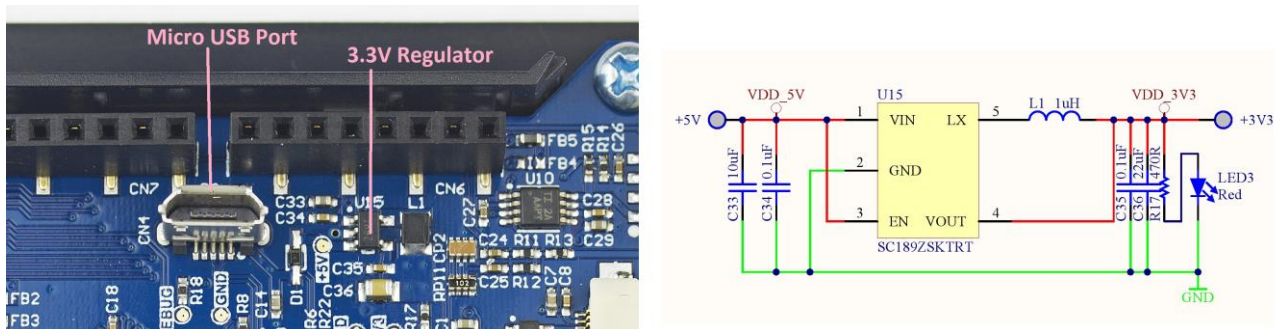
Figure 2 - Power Supply
