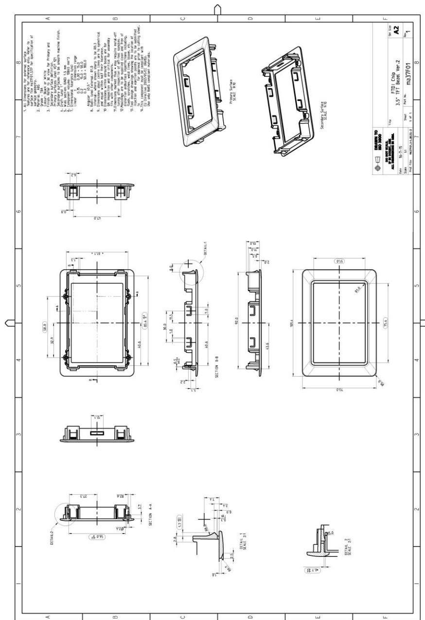
Figure 14 - Cle035 Bezel Drawing
