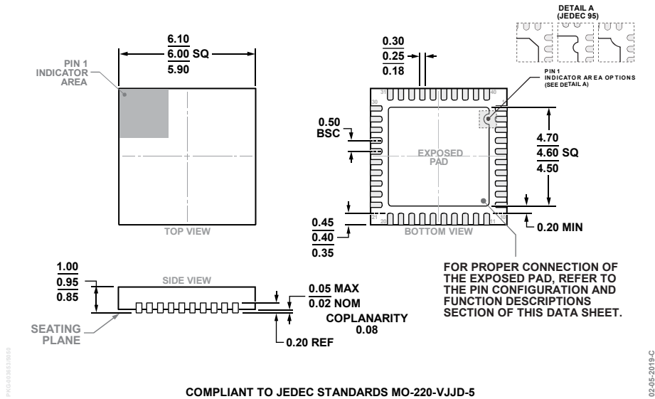
COMPLIANT TO JEDEC STANDARDS MO-220-VJJD-5 Figure 48. 40-Lead Lead Frame Chip Scale Package [LFCSP] 6 mm × 6 mm Body and 0.95 mm Package Height (CP-40-15) Dimensions shown in millimeters
