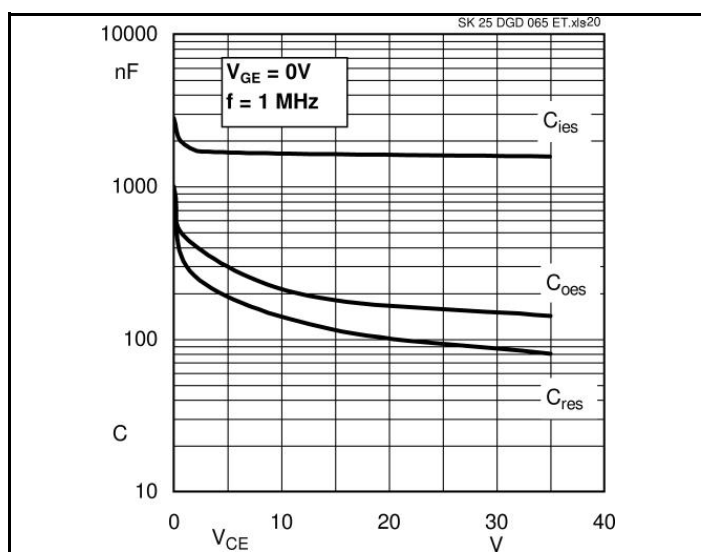
Fig. 20 Typical Capacitances vs. V_{CE}
