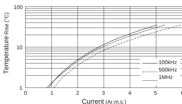
Ripple Current
