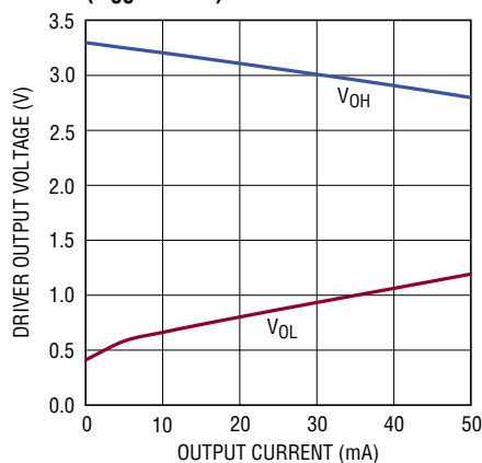
Y/Z Driver Output Low/High Voltage vs Output Current ( V_{CC} = 3.3\text{V} )
