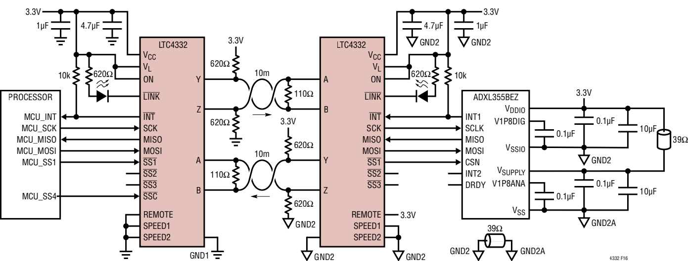
Figure 16. Extending an ADXL355BEZ Accelerometer for Remote Sensing
