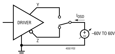
Figure 2. Driver Output Short-Circuit Current
