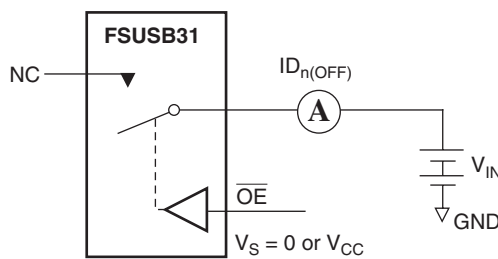
Figure 10. Off Leakage
