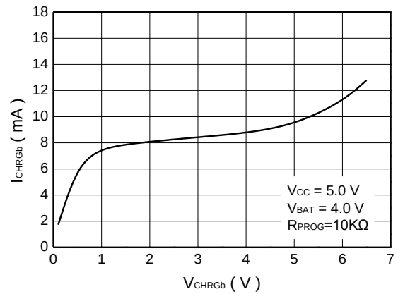
CHRGb Pin Current vs CHRGb Pin Voltage
