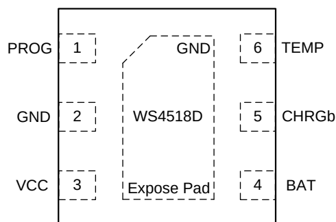
Pin configuration (Top view)
