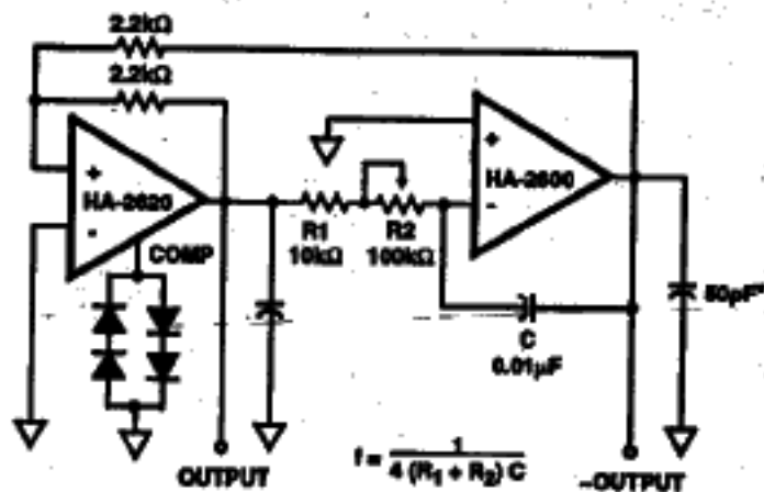
FIGURE 11. FUNCTION GENERATOR
