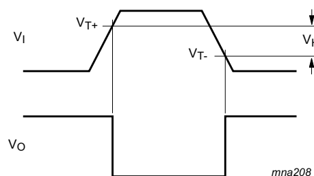
Fig 6. Definition of V_{T+} , V_{T-} , and V_H
