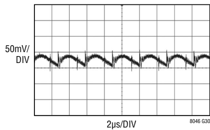
Output Ripple
