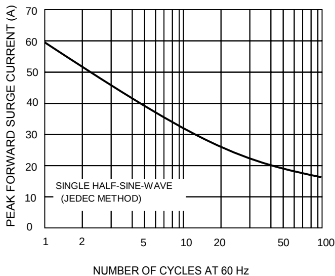
FIG.3 MAXIMUM NON-REPETITIVE
