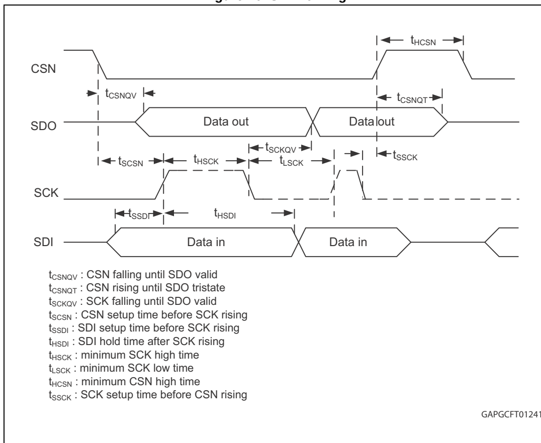
Figure 20. SPI – timing
