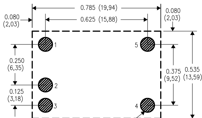
PC LAYOUT
