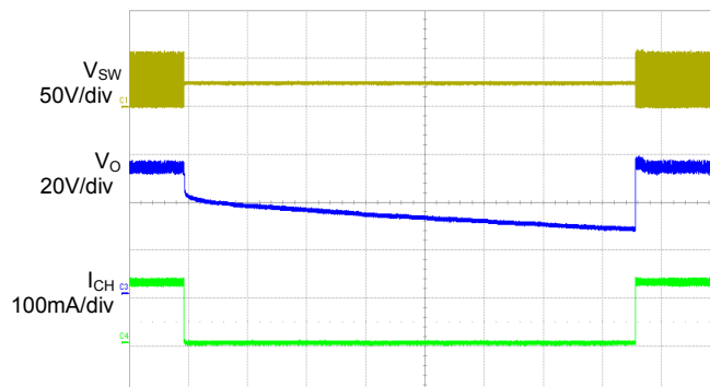
Overtemperature Protection
