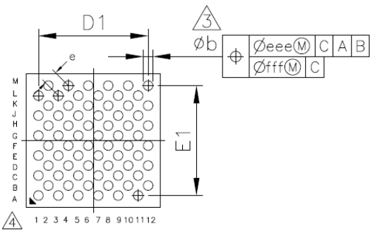
Figure 67: Bottom View
