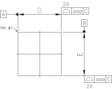
Figure 66: Top View
