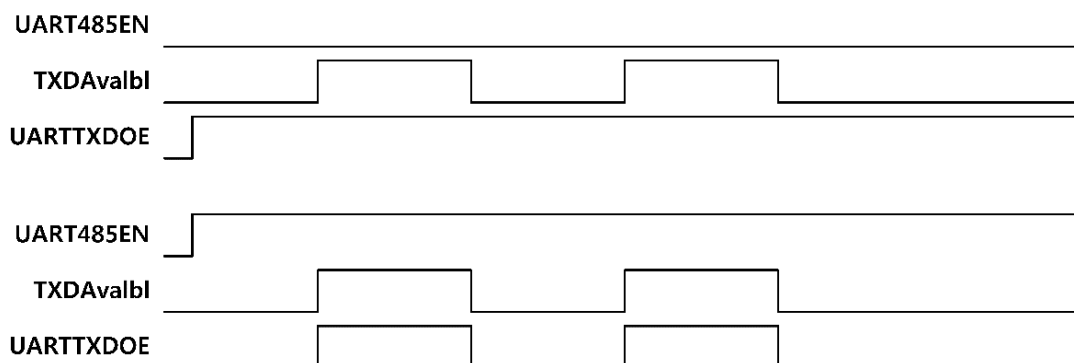
Figure 50: UARTTXDOE Output Signal for UART RS-485
