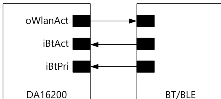
Figure 55: Bluetooth Coexistence Interface
