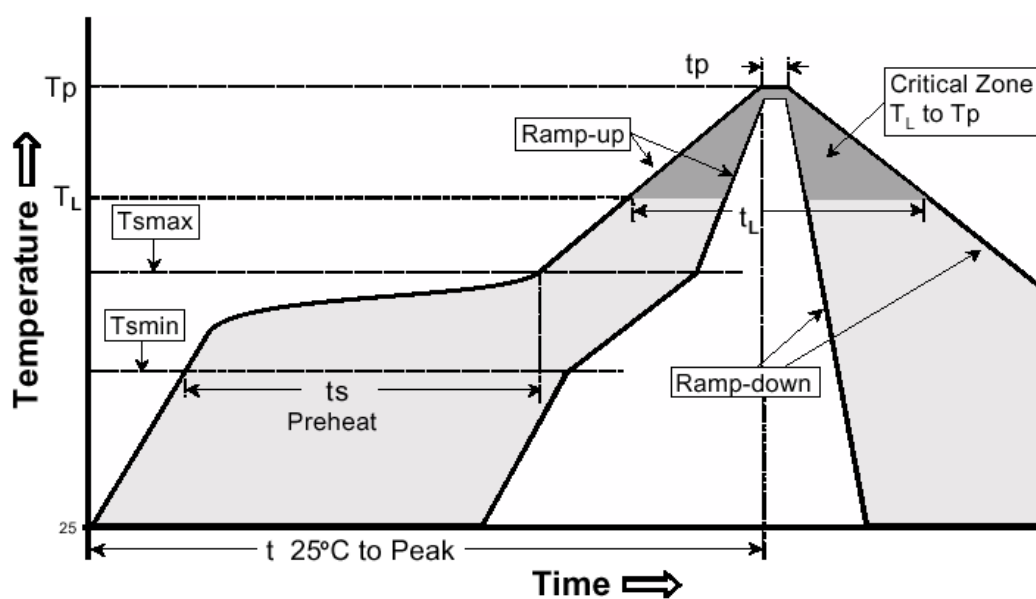
Figure 73: Reflow Condition
