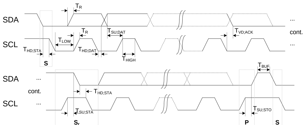
Figure 32: I2C Master Timing Diagram
