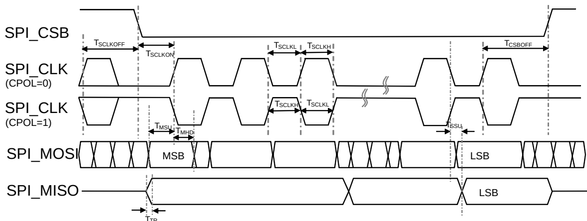
Figure 29: SPI Slave Timing Diagram
