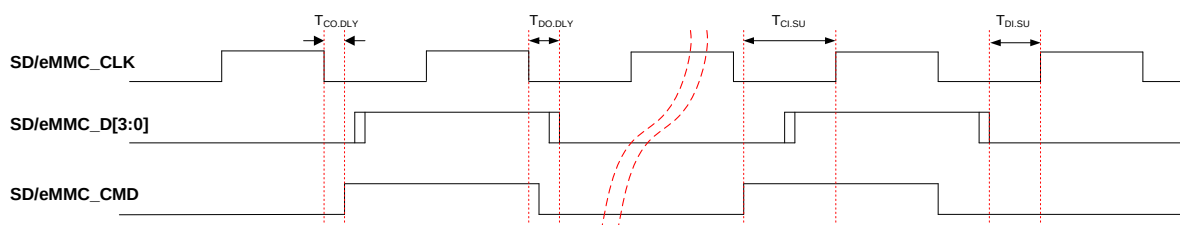
Figure 35: SD/eMMC Master Timing Diagram
