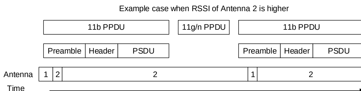
Figure 46: Antenna Switching Timing Diagram
