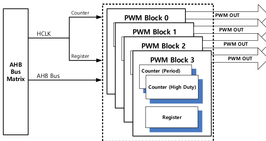
Figure 52: PWM Block Diagram
