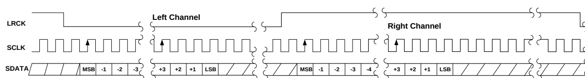
Figure 39: Left Justified Mode Timing Diagram
