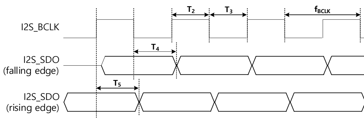
Figure 41: I2S Transmit Timing Diagram
