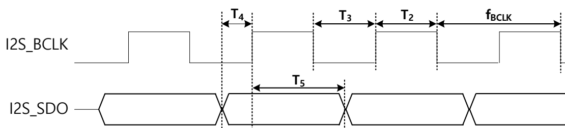
Figure 42: I2S Receive Timing Diagram
