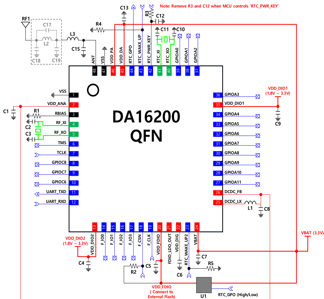
Figure 56: Typical Application – QFN, 3.3 V Flash
