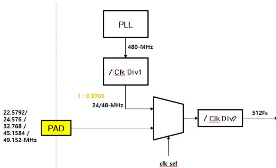
Figure 37: I2S Clock Scheme
