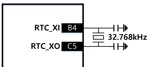
Figure 8: RTC Crystal Connections – fcCSP
