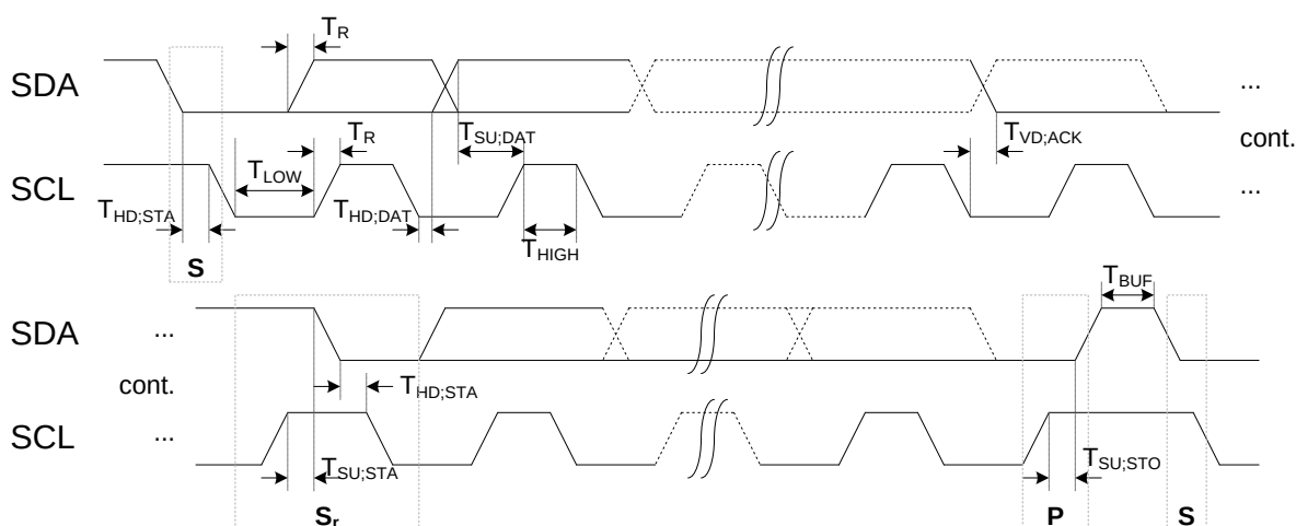
Figure 33: I2C Slave Timing Diagram
