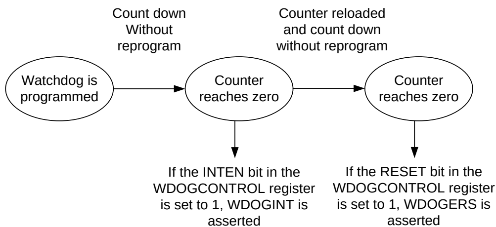
Figure 21: Watchdog Operation Flow Diagram
