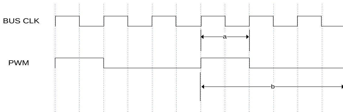
Figure 53: PWM Timing Diagram
