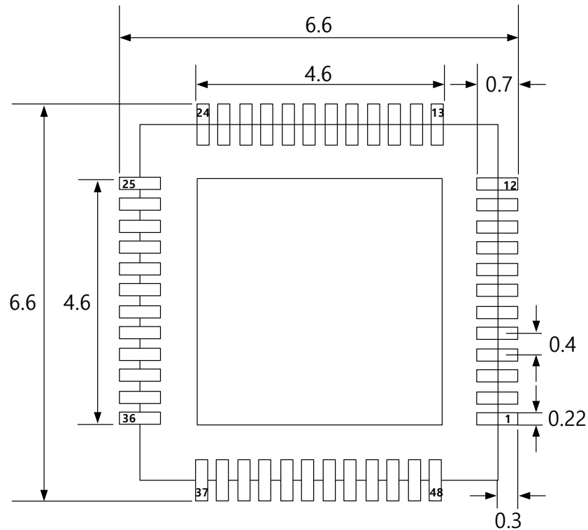
Figure 70: DA16200 48-Pin QFN Land Pattern
