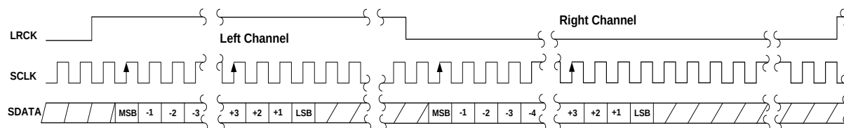
Figure 38: I2S Timing Diagram
