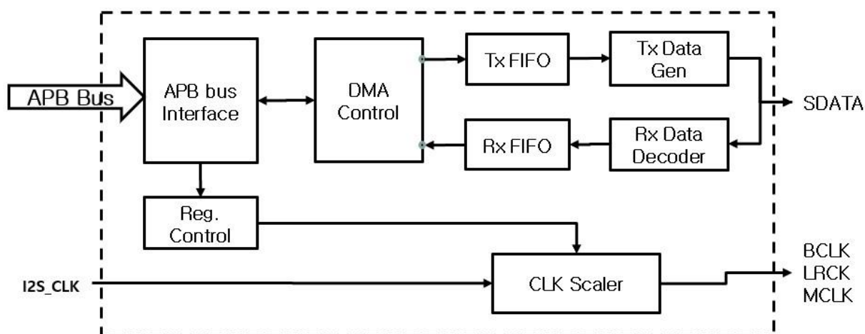
Figure 36: I2S Block Diagram
