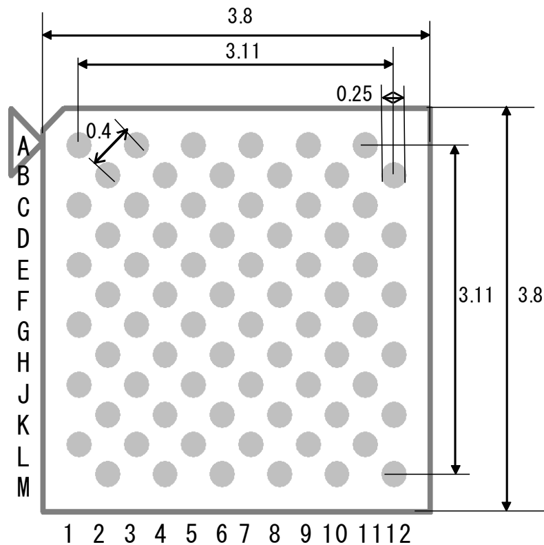
Figure 71: DA16200 72-Pin FcCSP Land Pattern
