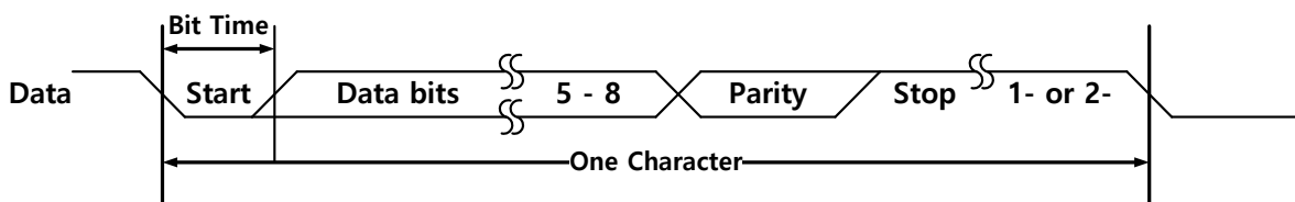
Figure 48: Serial Data Format
