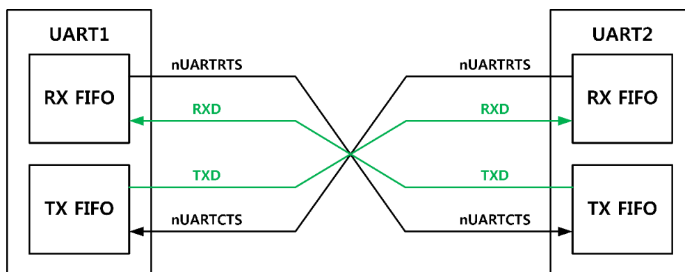
Figure 51: UART Hardware Flow Control
