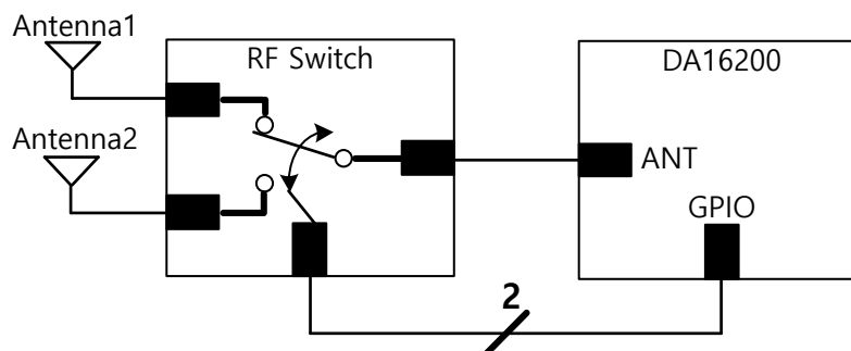
Figure 45: Antenna Switching Internal Block Diagram
