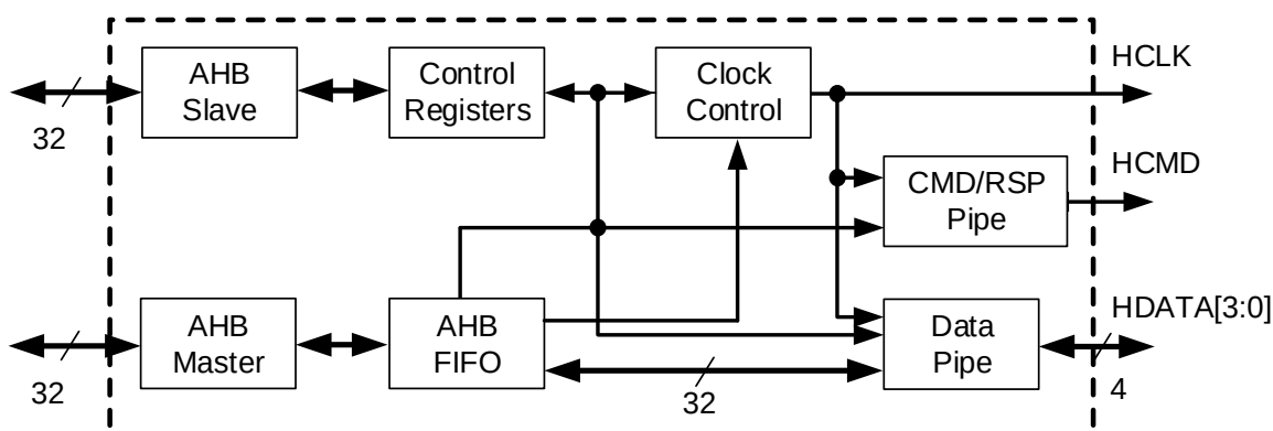
Figure 34: SD/eMMC Block Diagram
