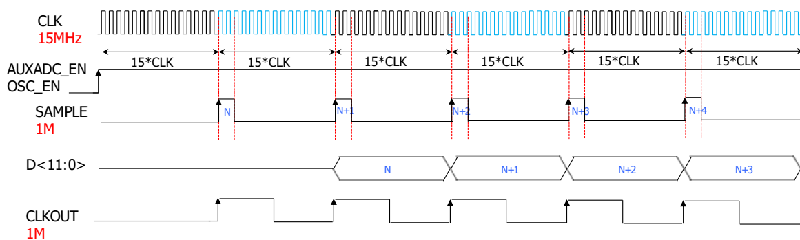
Figure 44: 12-bit ADC Timing Diagram
