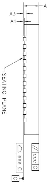
Figure 64: Side View
