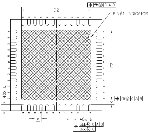
Figure 63: Bottom View
