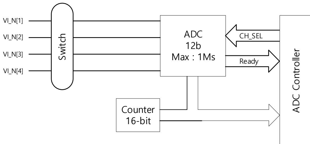
Figure 43: ADC Control Block Diagram
