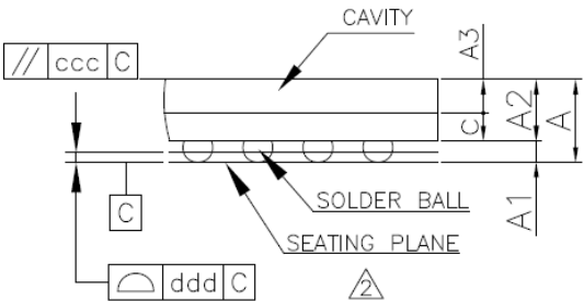
Figure 68: Side View
