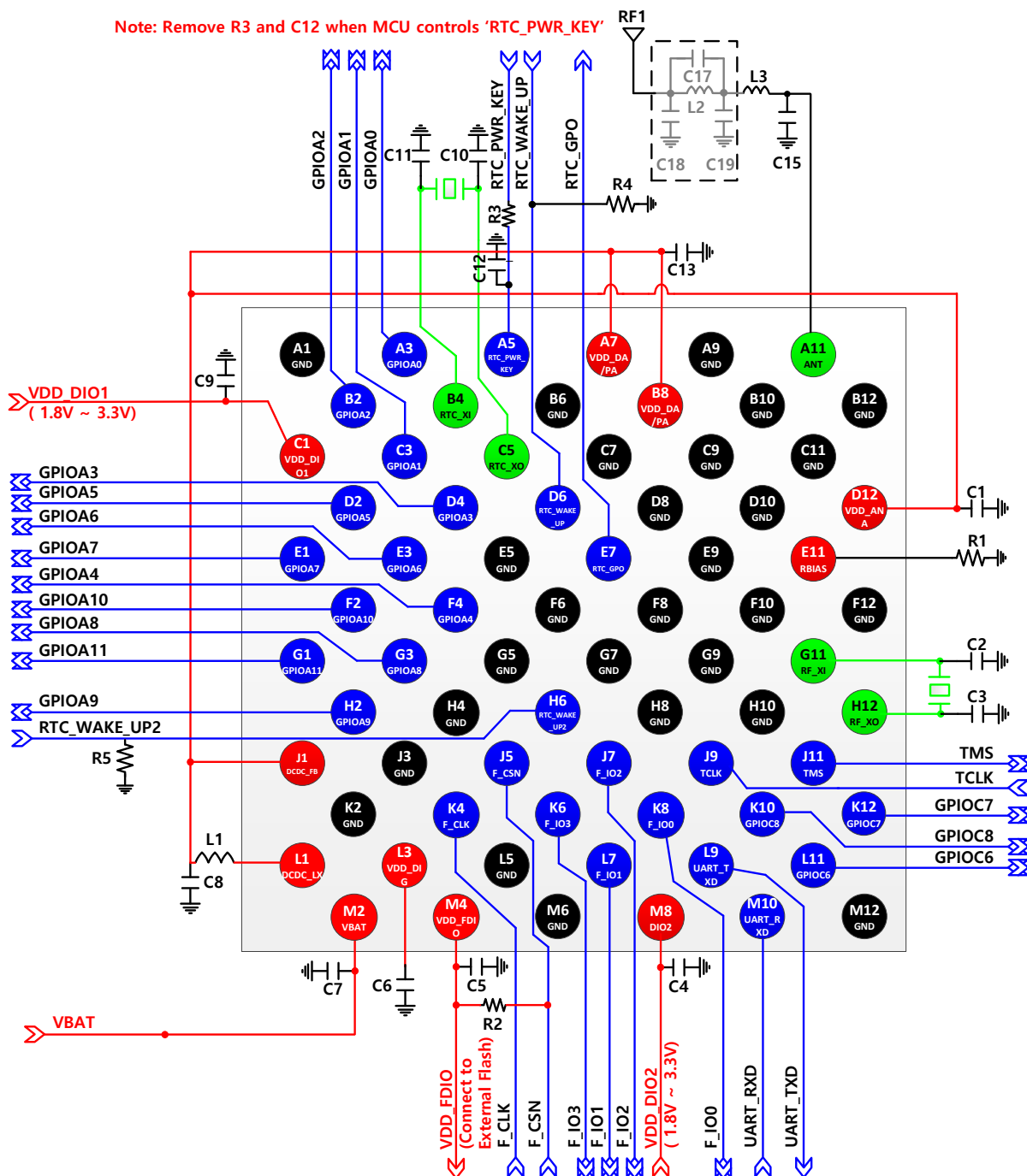
Figure 59: Typical Application – fcCSP, 1.8 V Flash, Low Power Mode
