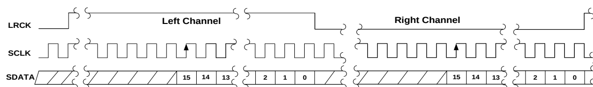
Figure 40: Right Justified Mode Timing Diagram
