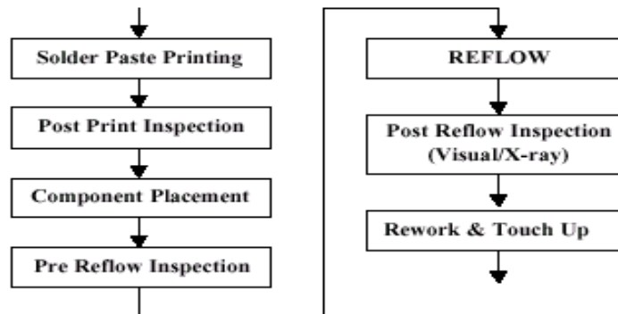
Figure 72: Typical PCB Mounting Process Flow
