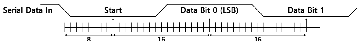
Figure 49: Receiver Serial Data Sampling Points
