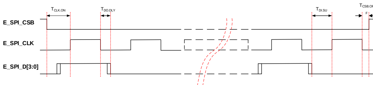
Figure 25: SPI Master Timing Diagram (Mode 0)
