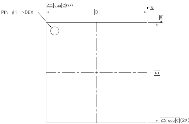
Figure 62: Top View
