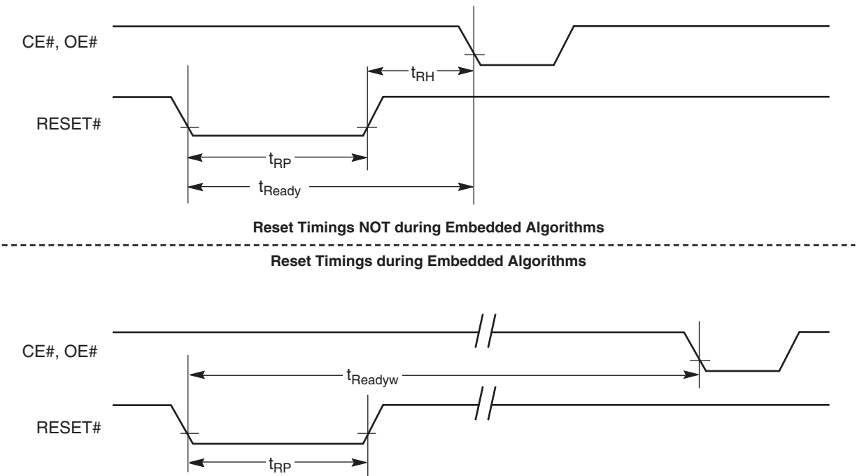
Figure 33. Reset Timings
