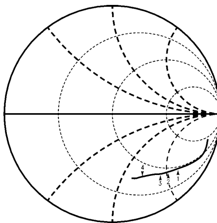
LMX2320/25 Input Impedance vs Frequency V_{CC} = 2.7V to 5.5V , f_{IN} = 500 MHz to 3000 MHz
