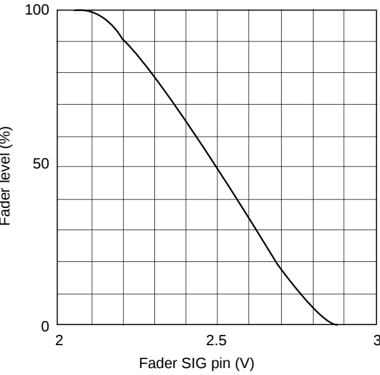
Chroma fader control characteristics
