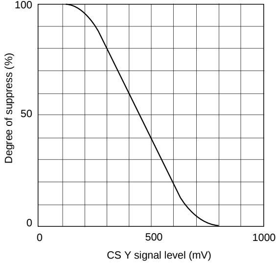
CS Y control characteristics
