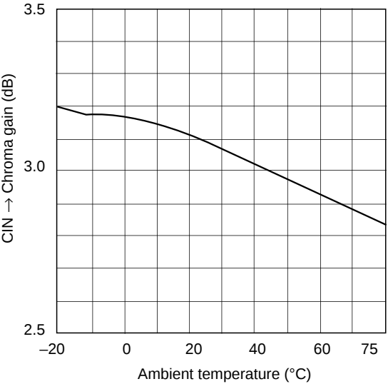
CIN → Chroma gain temperature characteristics
