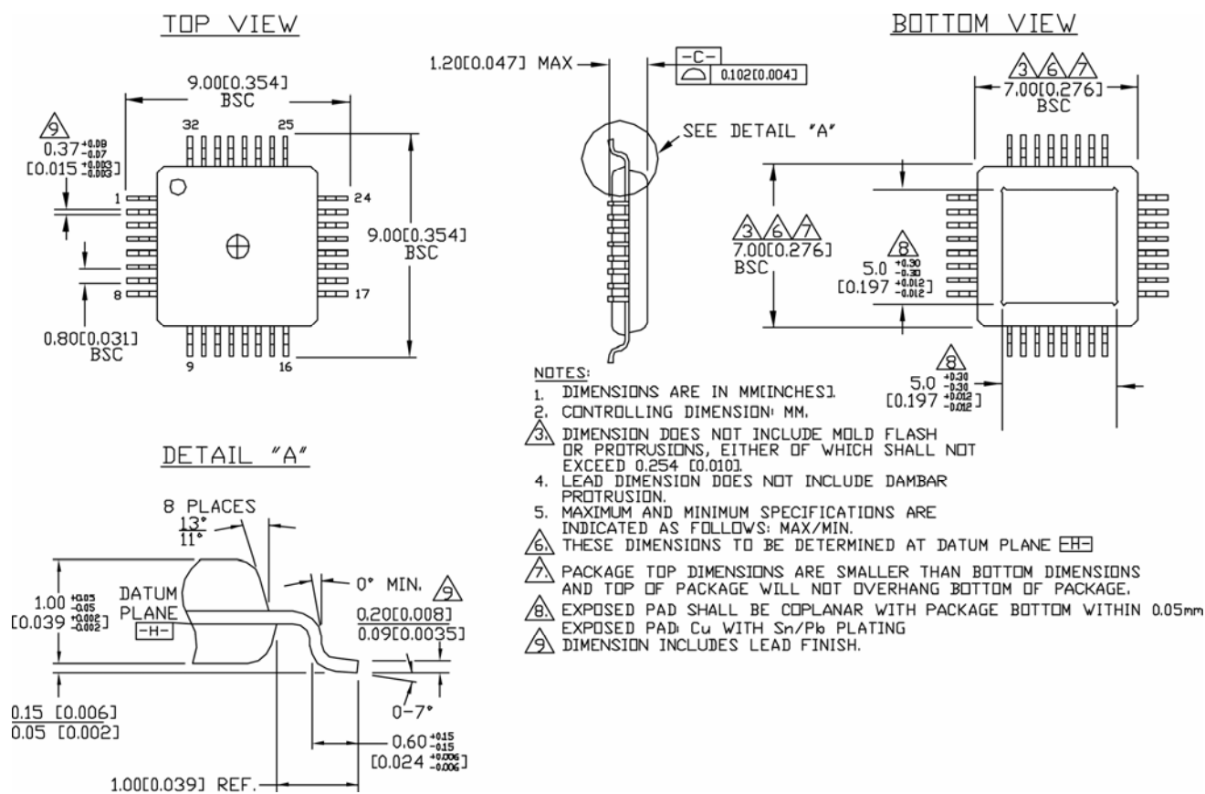
32-Pin Package Type (H32-1)
