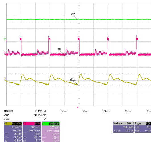
Figure 12: Charge Pump Off at I OUT = 1A
