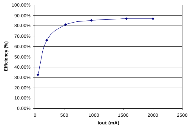
Fig.8 Output efficiency
