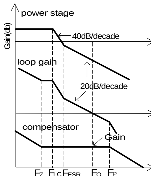
Figure 21 - Bode plot of Type II compensator
