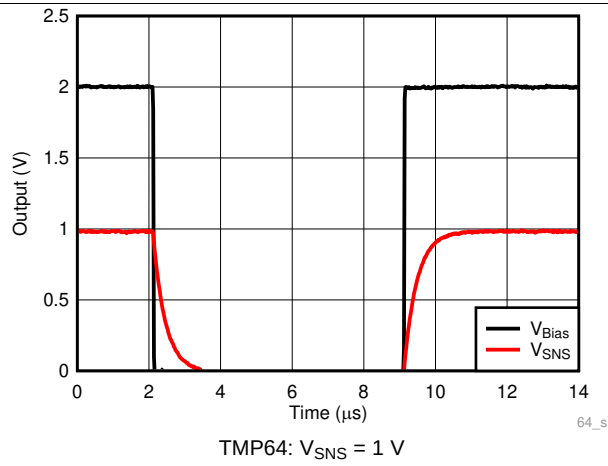
Figure 7. Step Response
