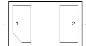
DEC Package 2-Pin X1SON Bottom View
