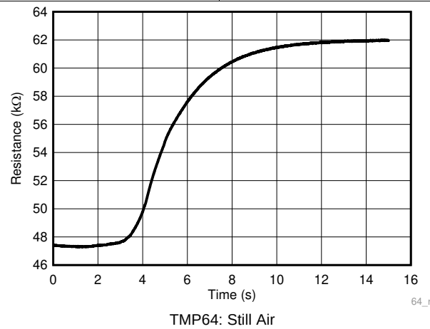
Figure 9. Thermal Response Time
