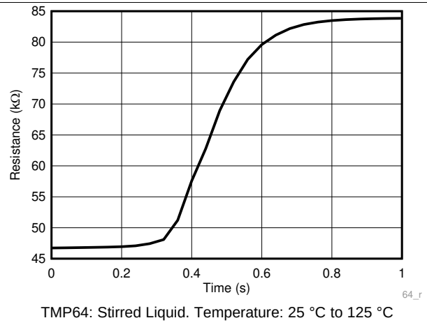
Figure 8. Thermal Response Time
