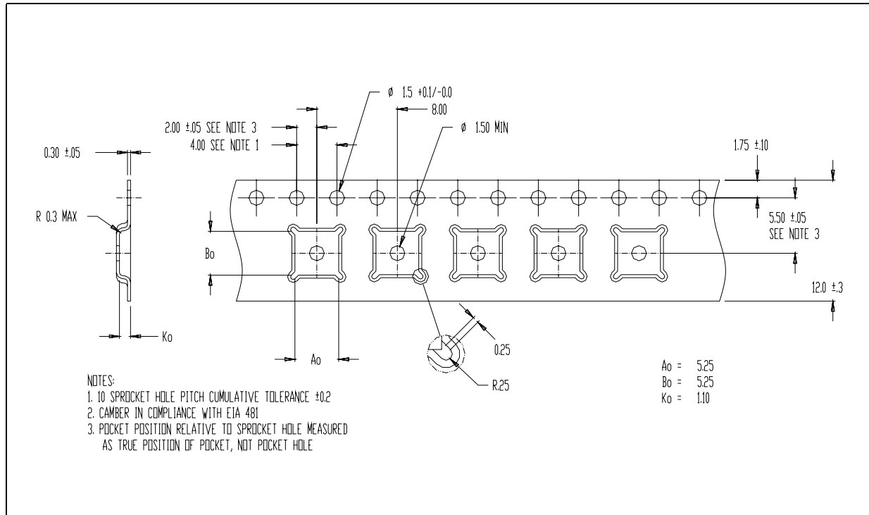
Figure 15. PowerFLAT™ Tape &amp; Reel
