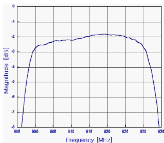
Frequency Response
