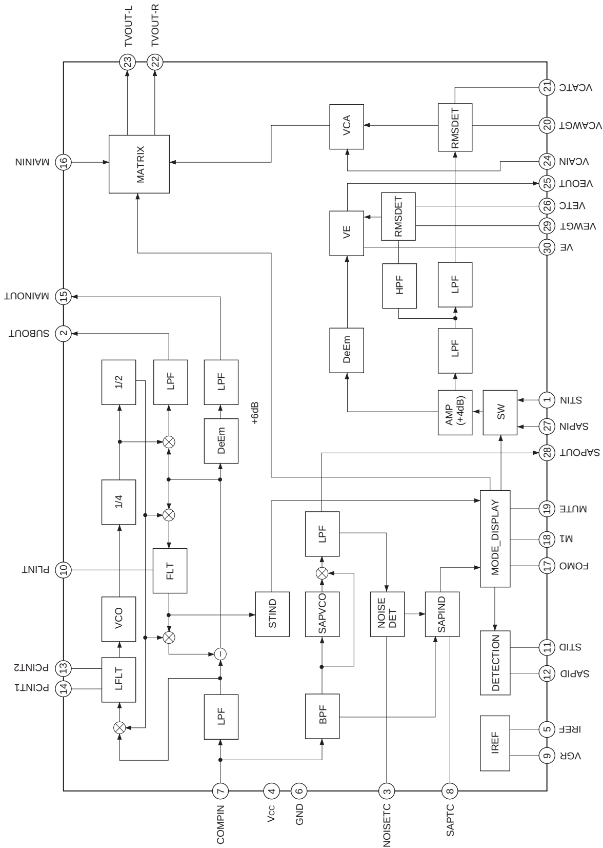
Block Diagram
