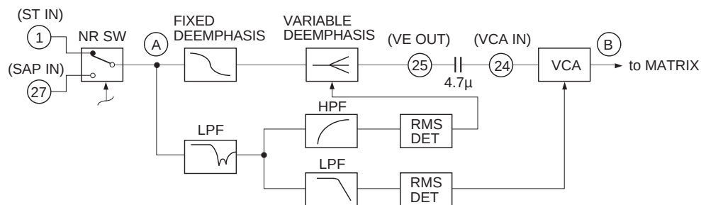
Fig 4. dbx-TV block
