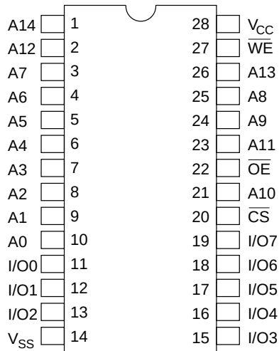
HM62W256LFP Series
