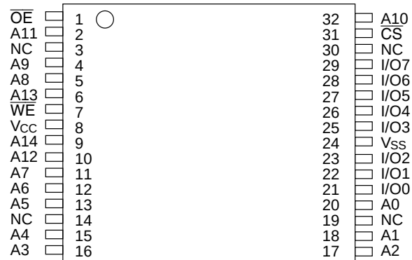
HM62W256LT Series
