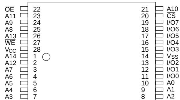
HM62W256LTM Series
