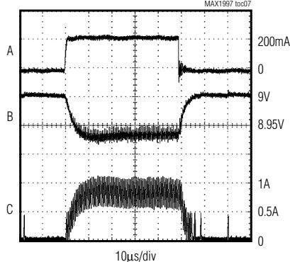
STEP-UP REGULATOR LOAD TRANSIENT RESPONSE (WITHOUT LAG COMPENSATION, FIGURE 1)
